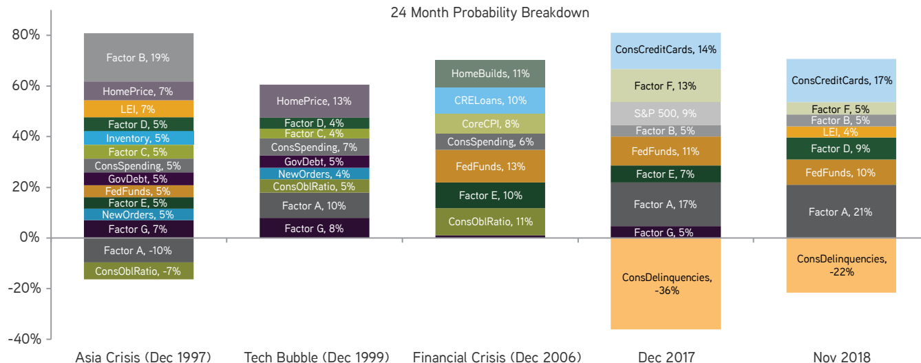
24 Month Probability Breakdown
